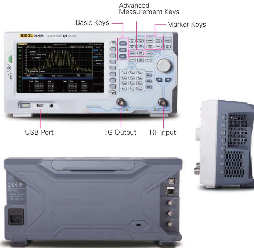
Product Dimensions: Width X Height X Depth = 361.6 mm x 178.8 mm x 128 mm
